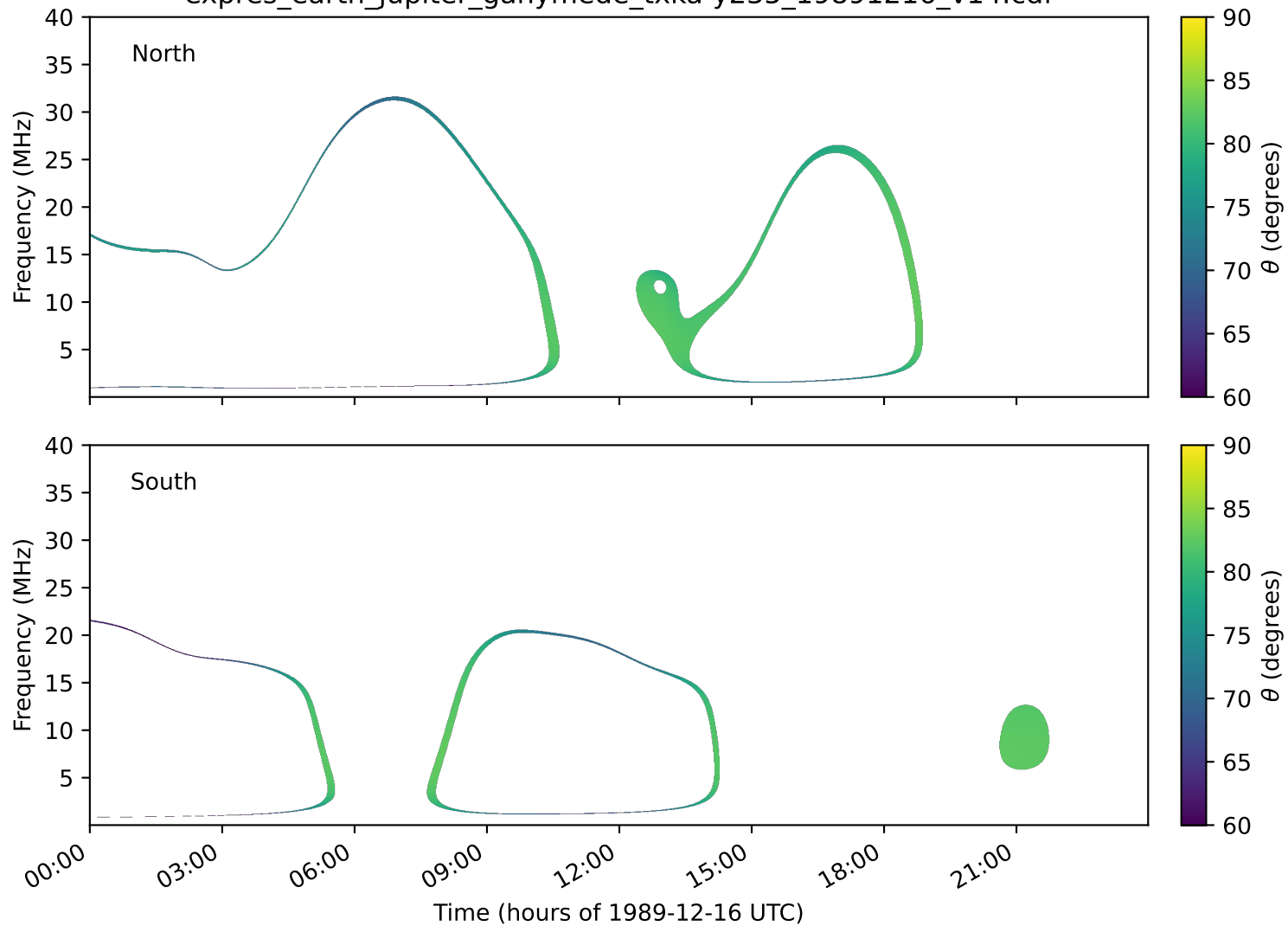
expres_earth_jupiter_ganymede_txka-y235_19891216_v14.cdf
