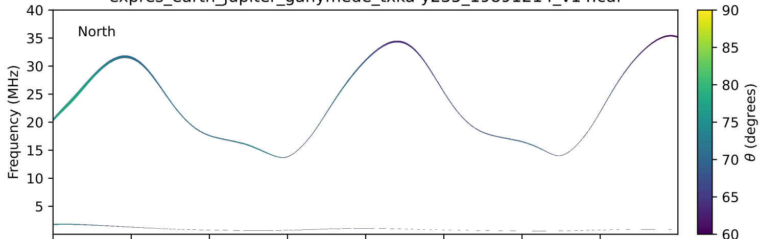
expres_earth_jupiter_ganymede_txka-y235_19891214_v14.cdf
