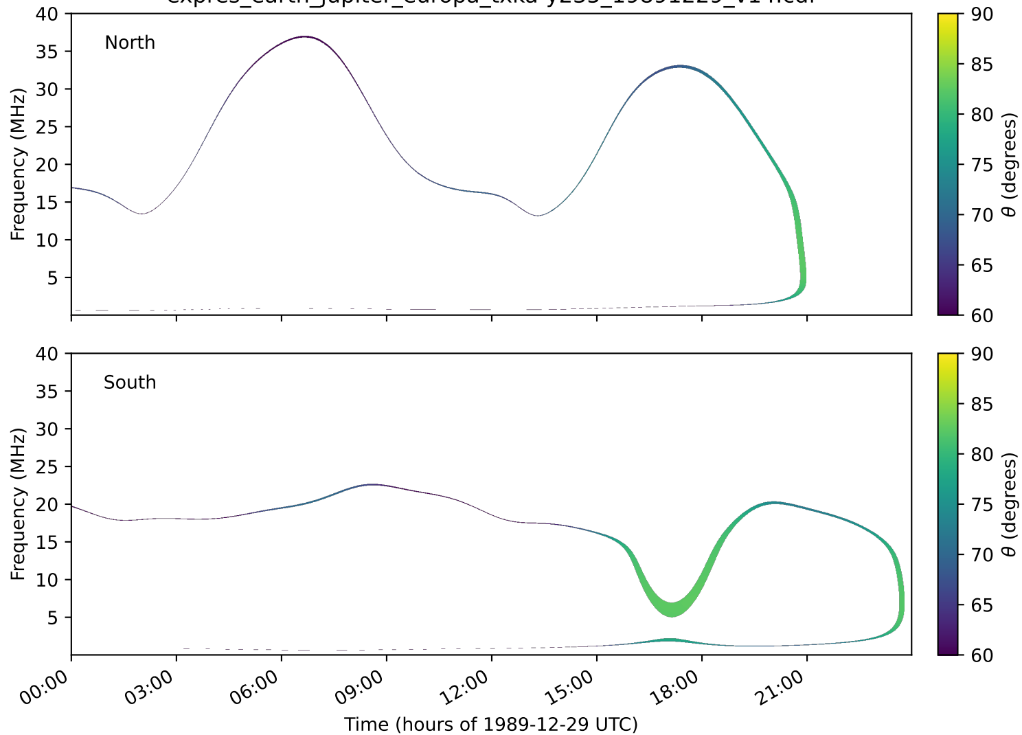
expres_earth_jupiter_europa_txka-y235_19891229_v14.cdf
