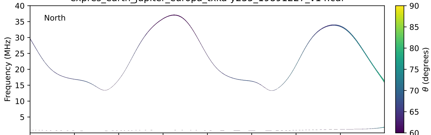
expres_earth_jupiter_europa_txka-y235_19891227_v14.cdf
