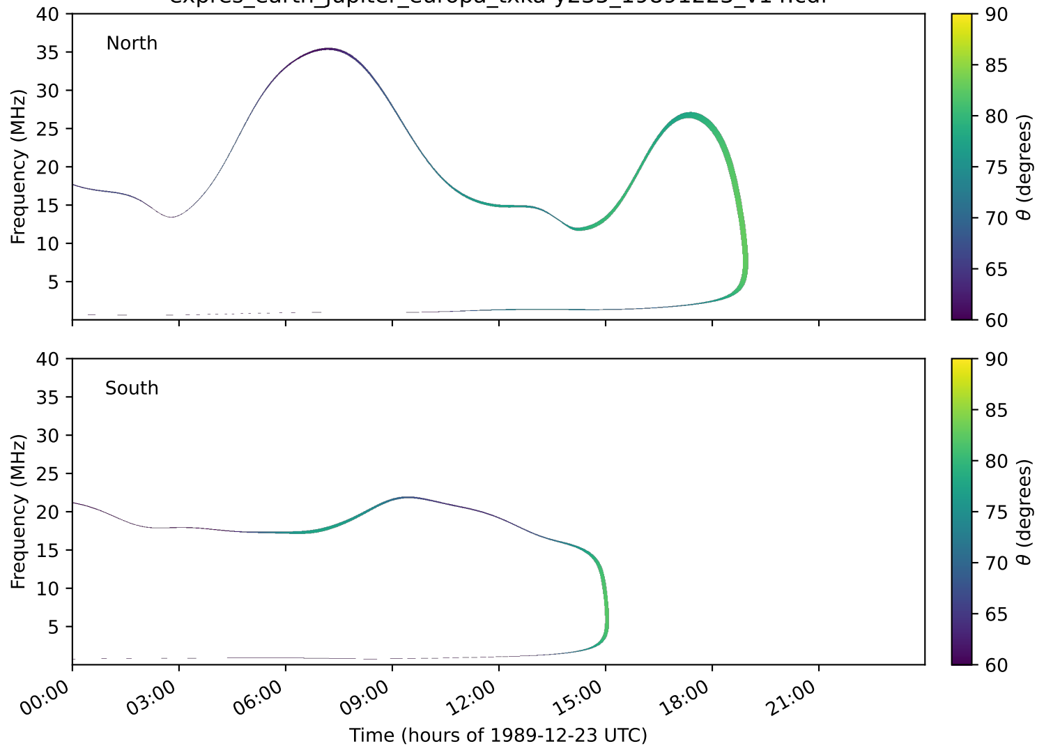
expres_earth_jupiter_europa_txka-y235_19891223_v14.cdf
