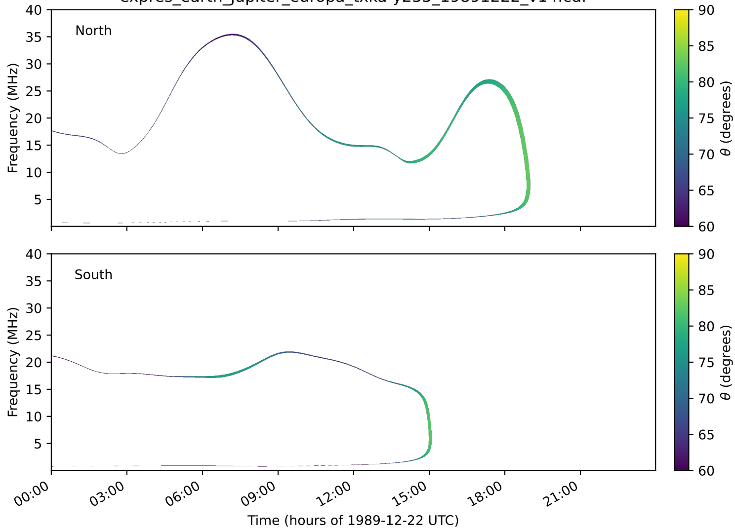
expres_earth_jupiter_europa_txka-y235_19891222_v14.cdf
