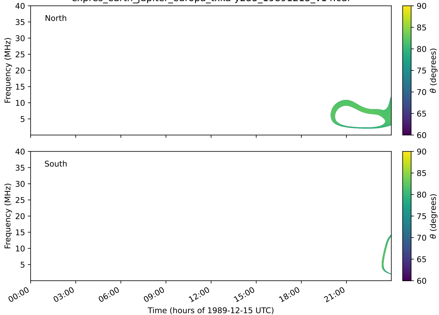
expres_earth_jupiter_europa_txka-y235_19891215_v14.cdf
