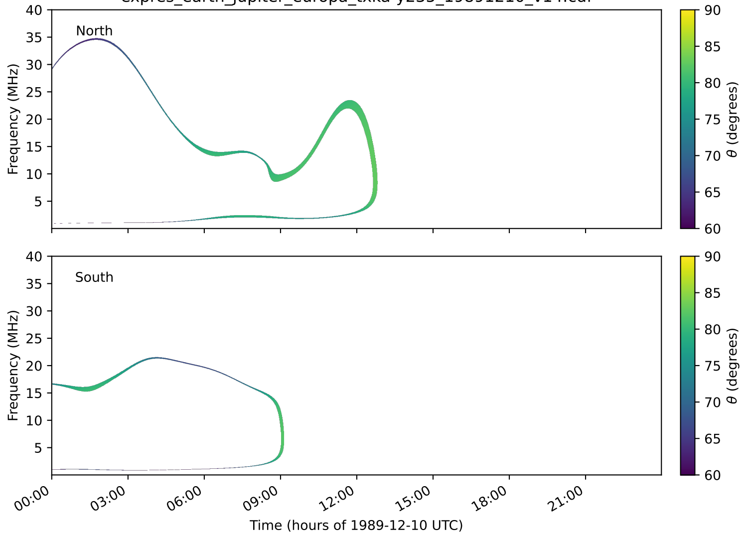
expres_earth_jupiter_europa_txka-y235_19891210_v14.cdf
