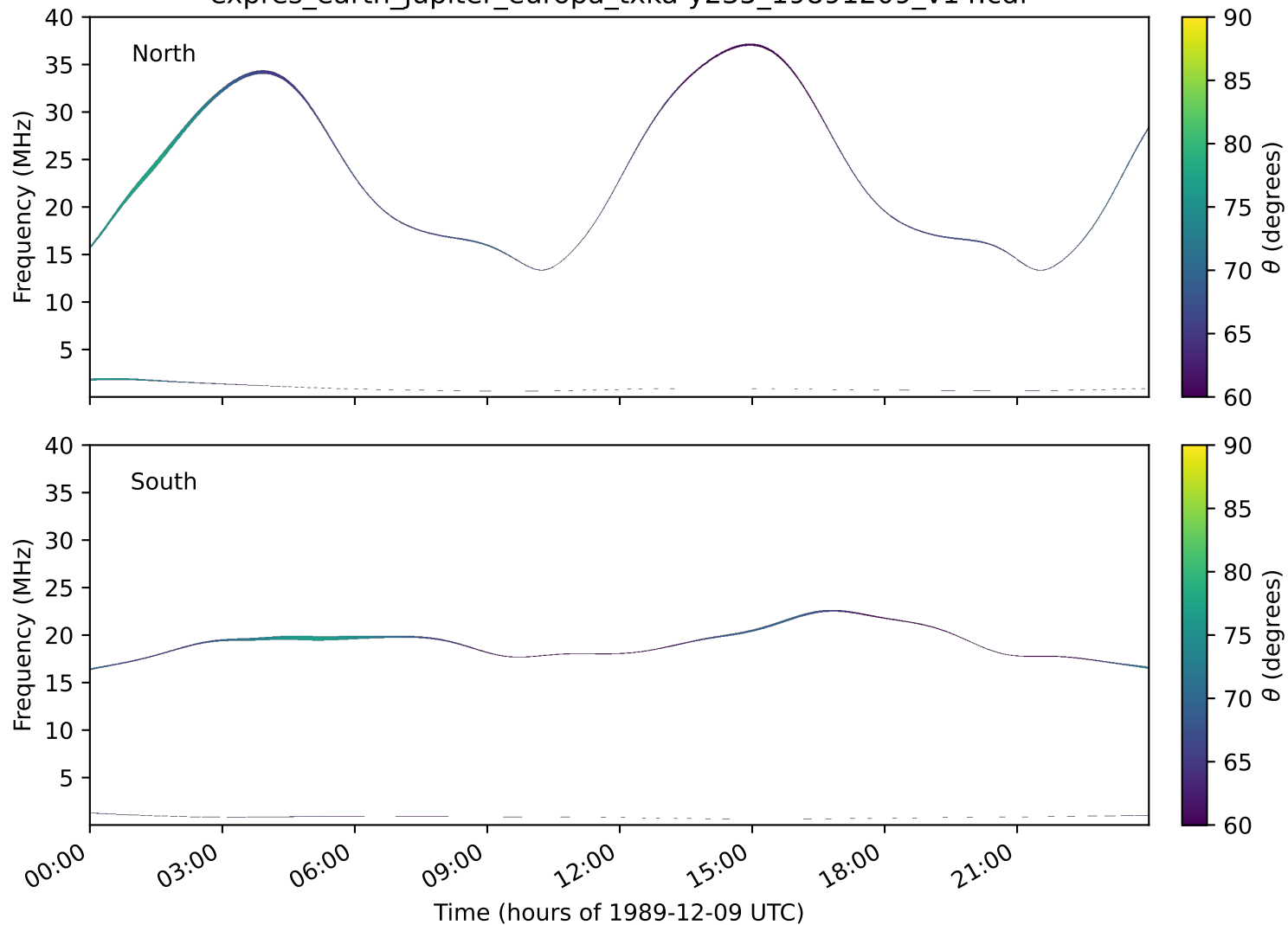
expres_earth_jupiter_europa_txka-y235_19891209_v14.cdf
