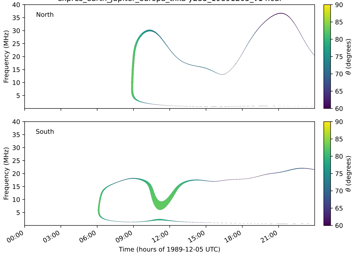
expres_earth_jupiter_europa_txka-y235_19891205_v14.cdf
