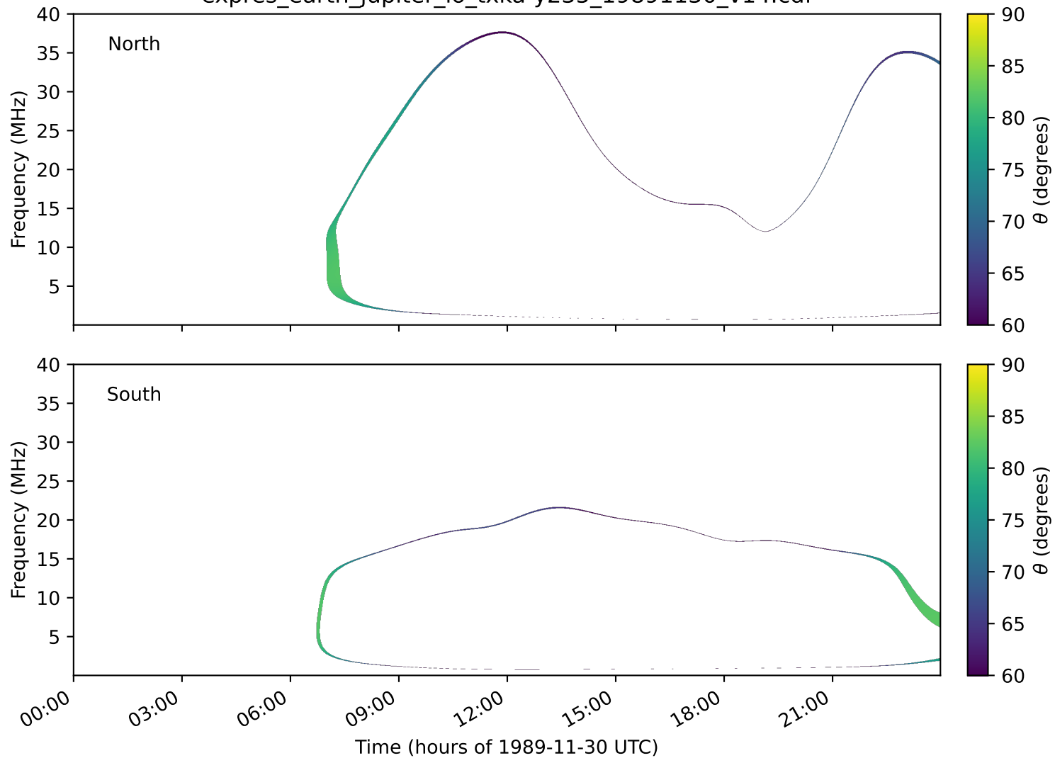
expres_earth_jupiter_io_txka-y235_19891130_v14.cdf
