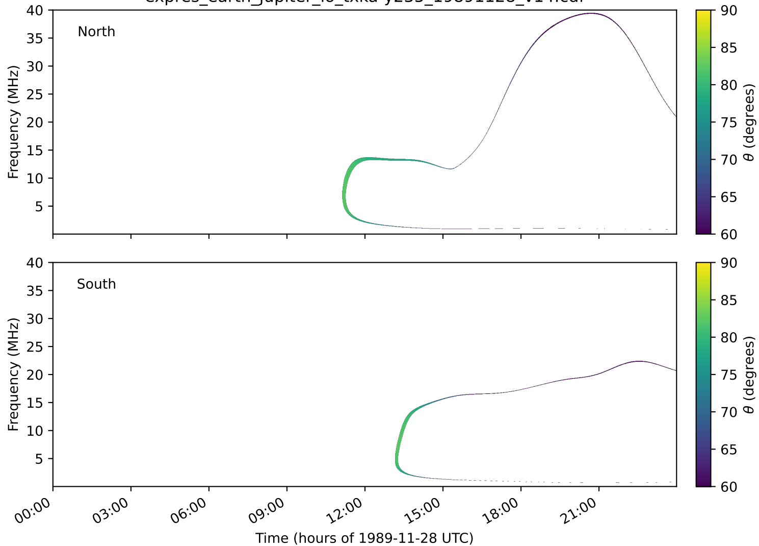
expres_earth_jupiter_io_txka-y235_19891128_v14.cdf
