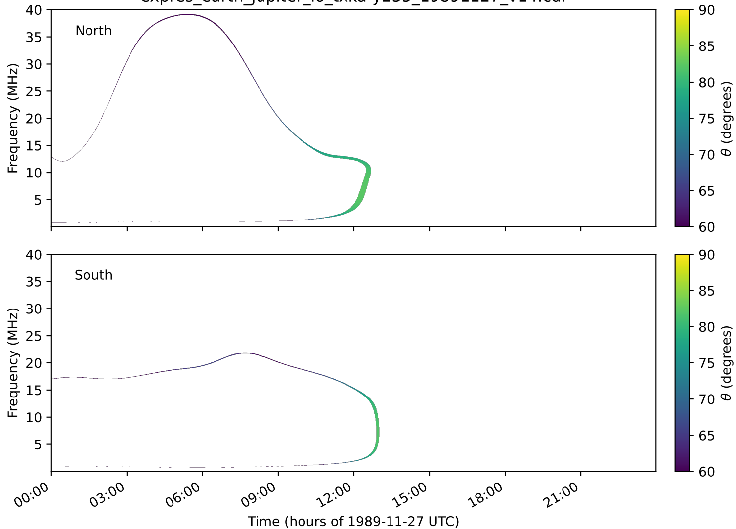
expres_earth_jupiter_io_txka-y235_19891127_v14.cdf
