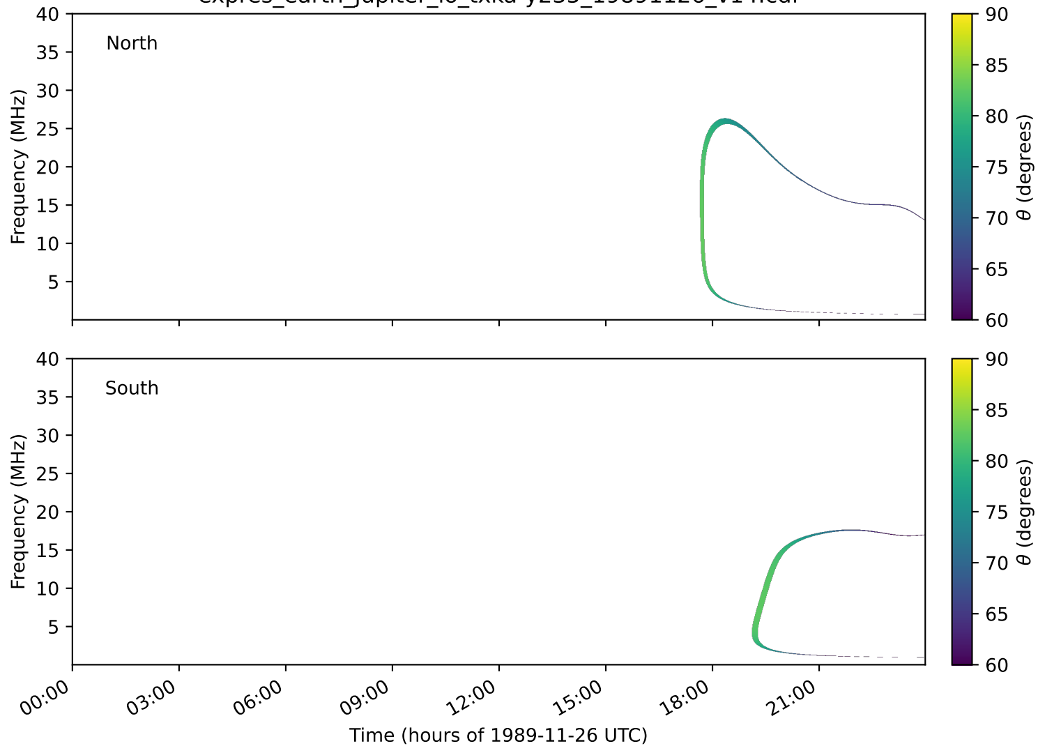
expres_earth_jupiter_io_txka-y235_19891126_v14.cdf
