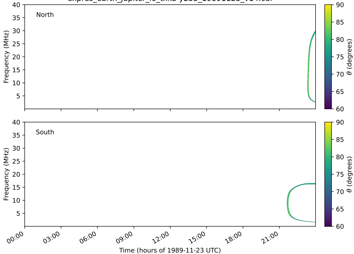
expres_earth_jupiter_io_txka-y235_19891123_v14.cdf
