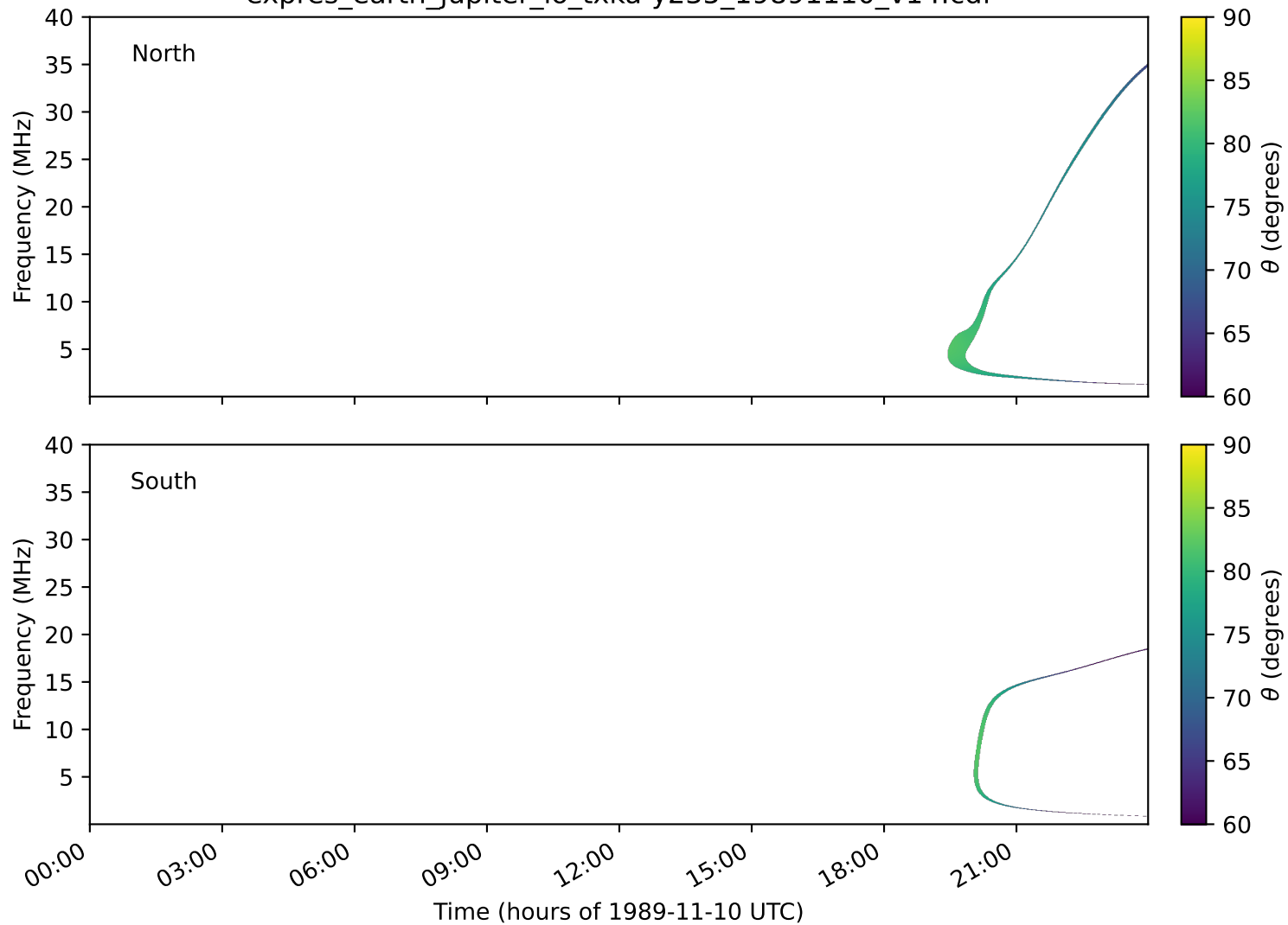
expres_earth_jupiter_io_txka-y235_19891110_v14.cdf
