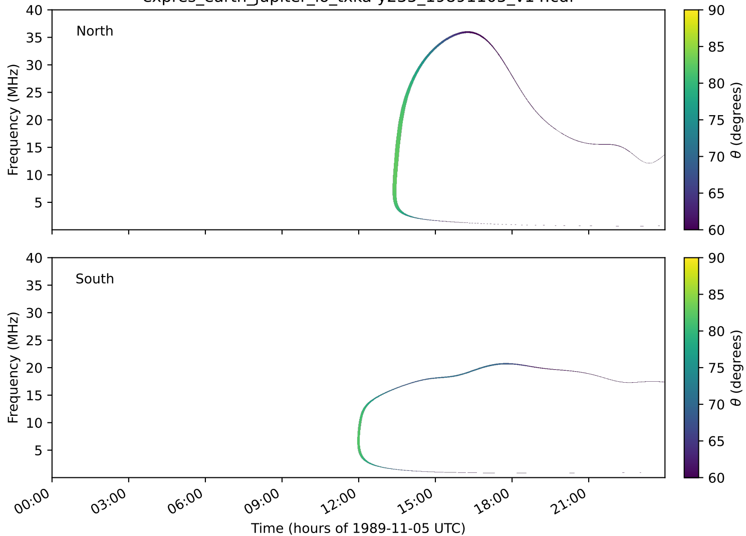
expres_earth_jupiter_io_txka-y235_19891105_v14.cdf
