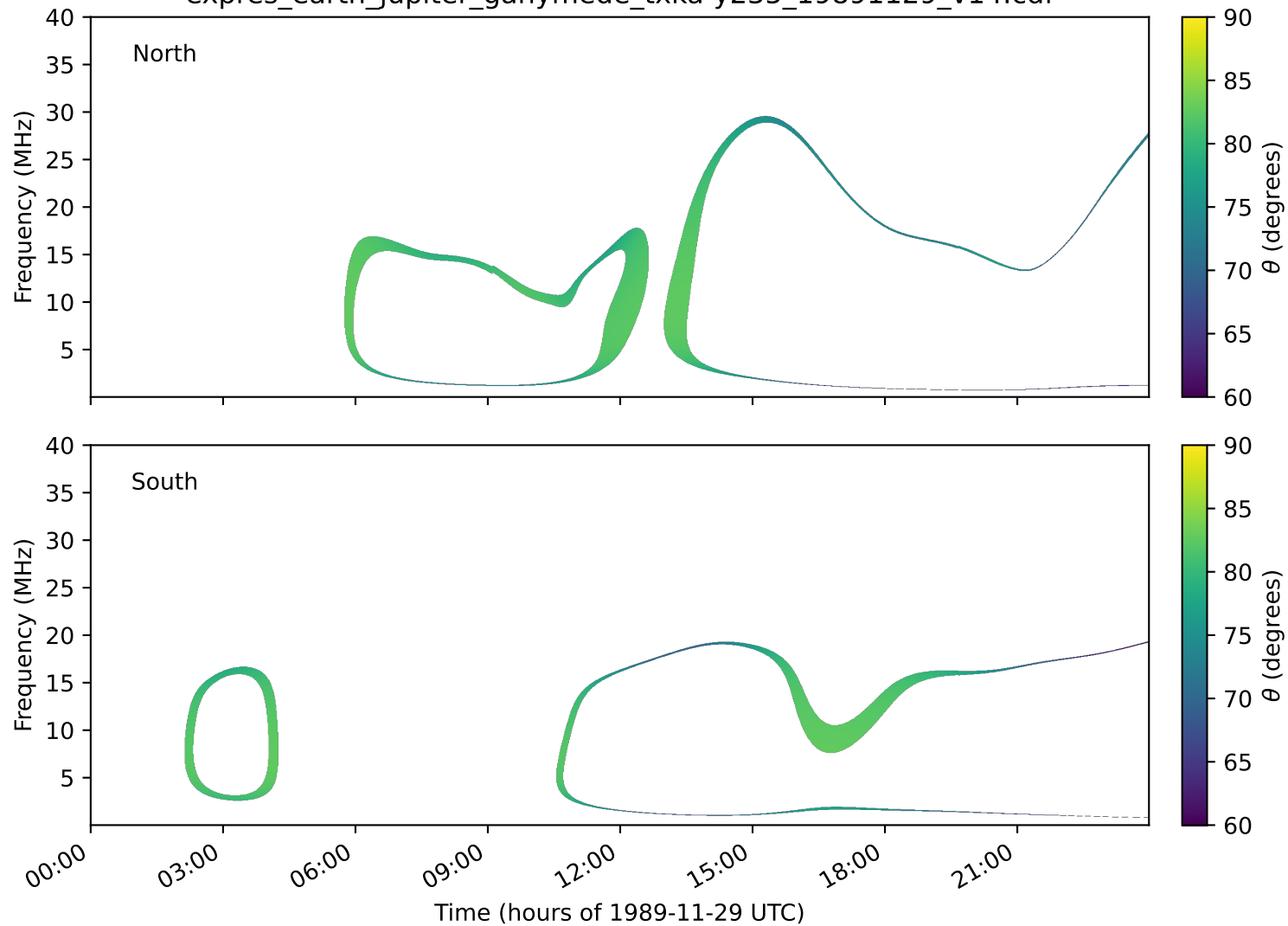
expres_earth_jupiter_ganymede_txka-y235_19891129_v14.cdf
