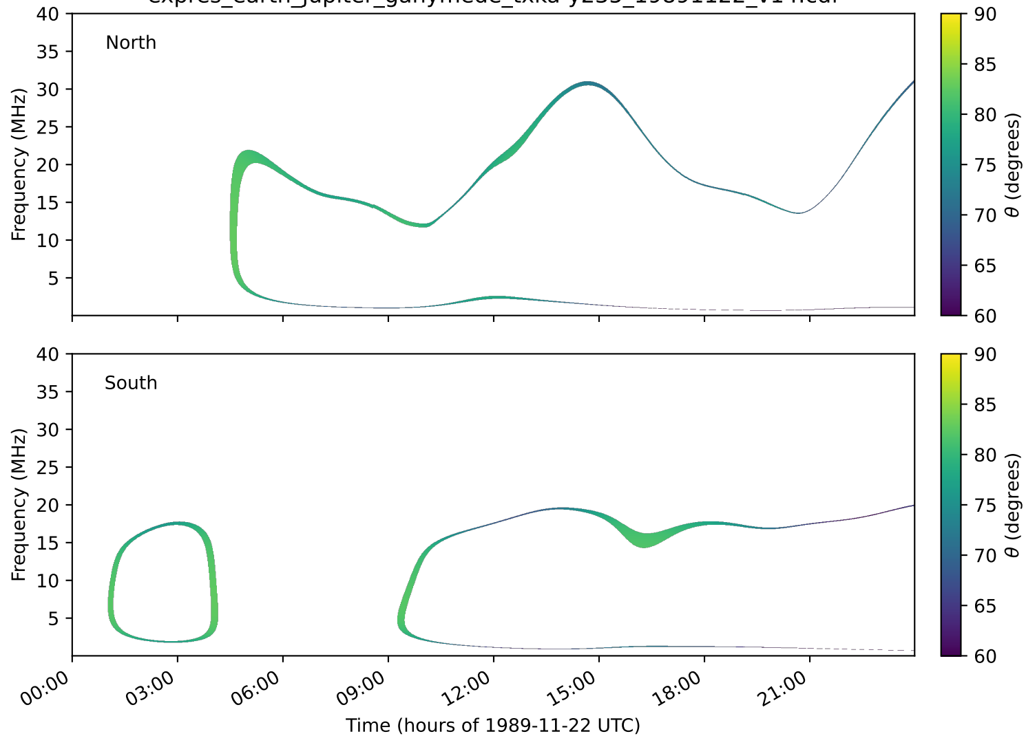
expres_earth_jupiter_ganymede_txka-y235_19891122_v14.cdf
