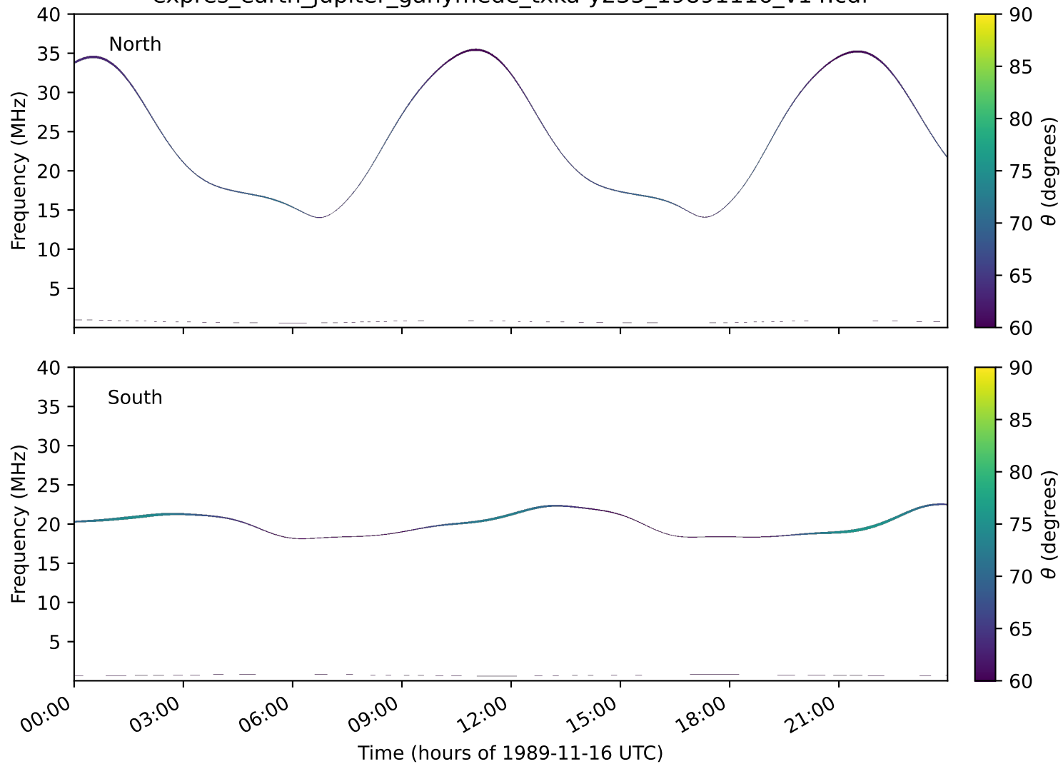
expres_earth_jupiter_ganymede_txka-y235_19891116_v14.cdf
