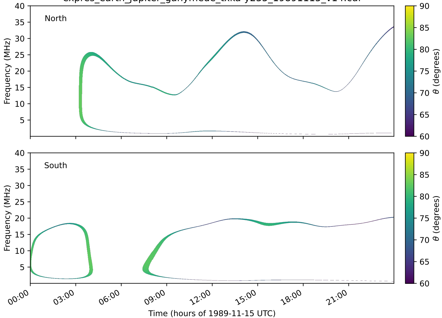
expres_earth_jupiter_ganymede_txka-y235_19891115_v14.cdf
