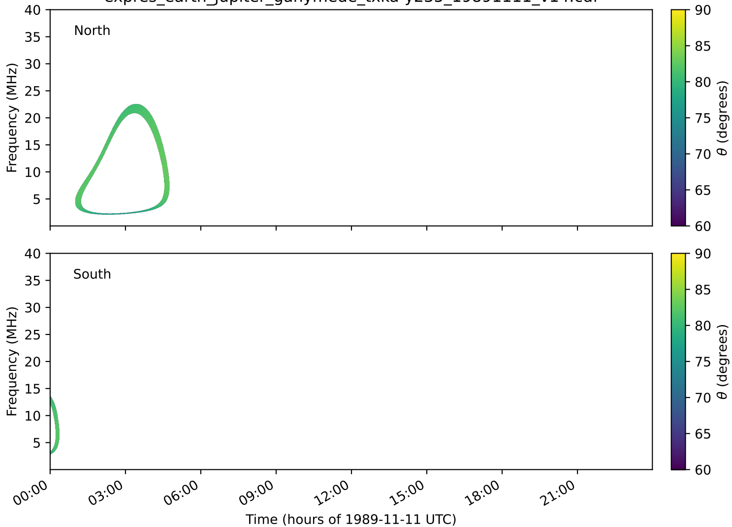
expres_earth_jupiter_ganymede_txka-y235_19891111_v14.cdf
