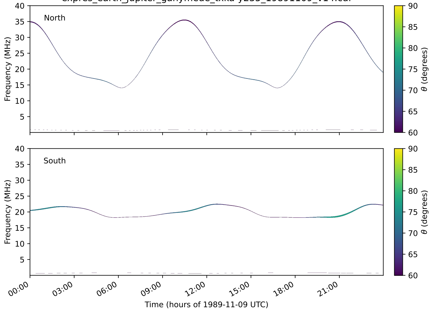
expres_earth_jupiter_ganymede_txka-y235_19891109_v14.cdf
