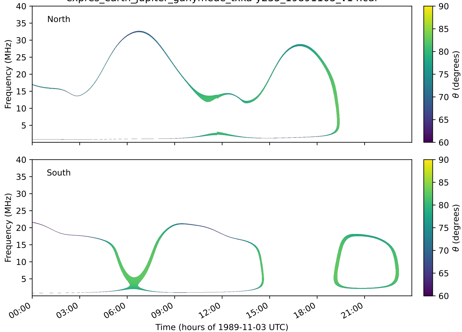
expres_earth_jupiter_ganymede_txka-y235_19891103_v14.cdf
