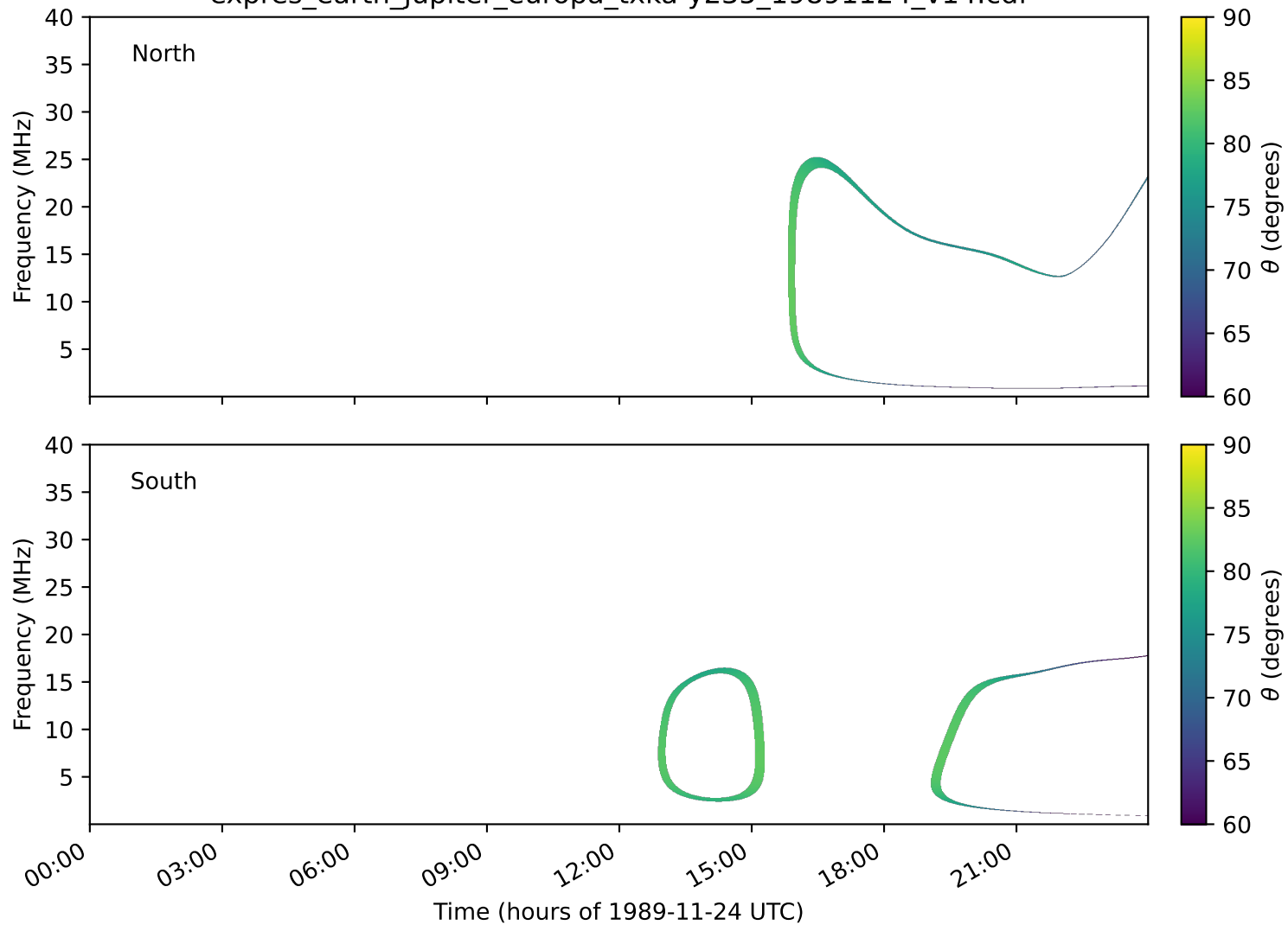
expres_earth_jupiter_europa_txka-y235_19891124_v14.cdf
