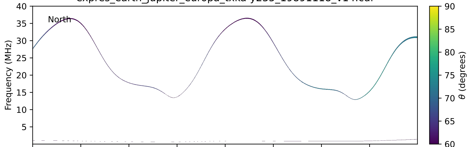
expres_earth_jupiter_europa_txka-y235_19891118_v14.cdf
