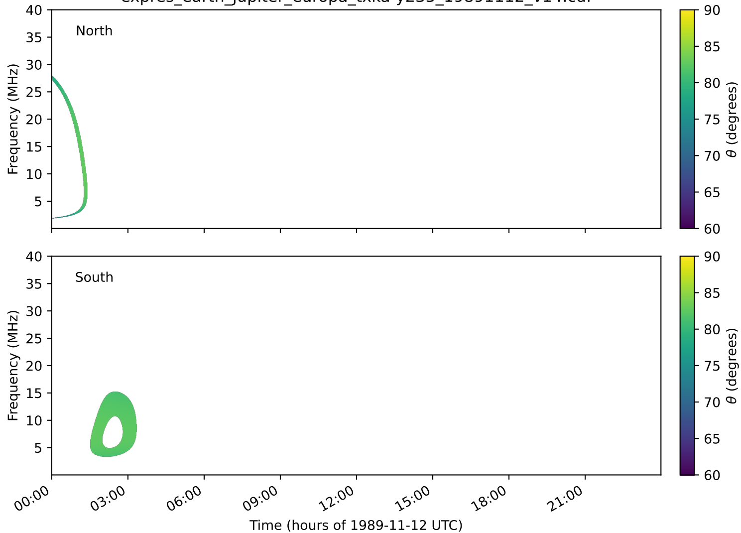
expres_earth_jupiter_europa_txka-y235_19891112_v14.cdf
