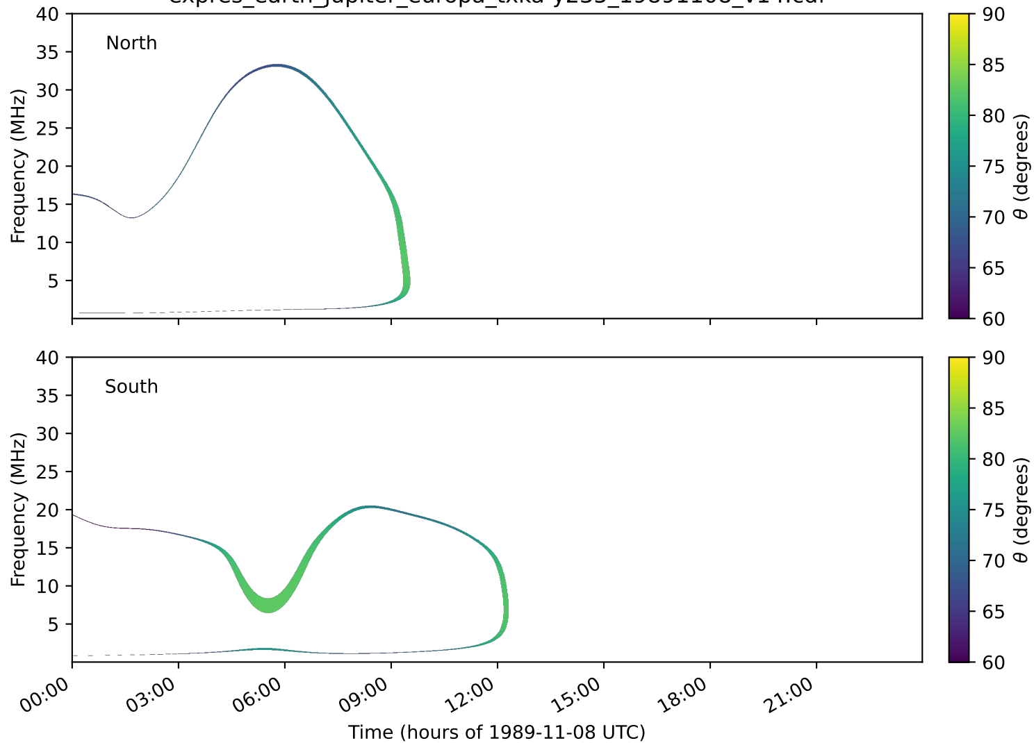
expres_earth_jupiter_europa_txka-y235_19891108_v14.cdf
