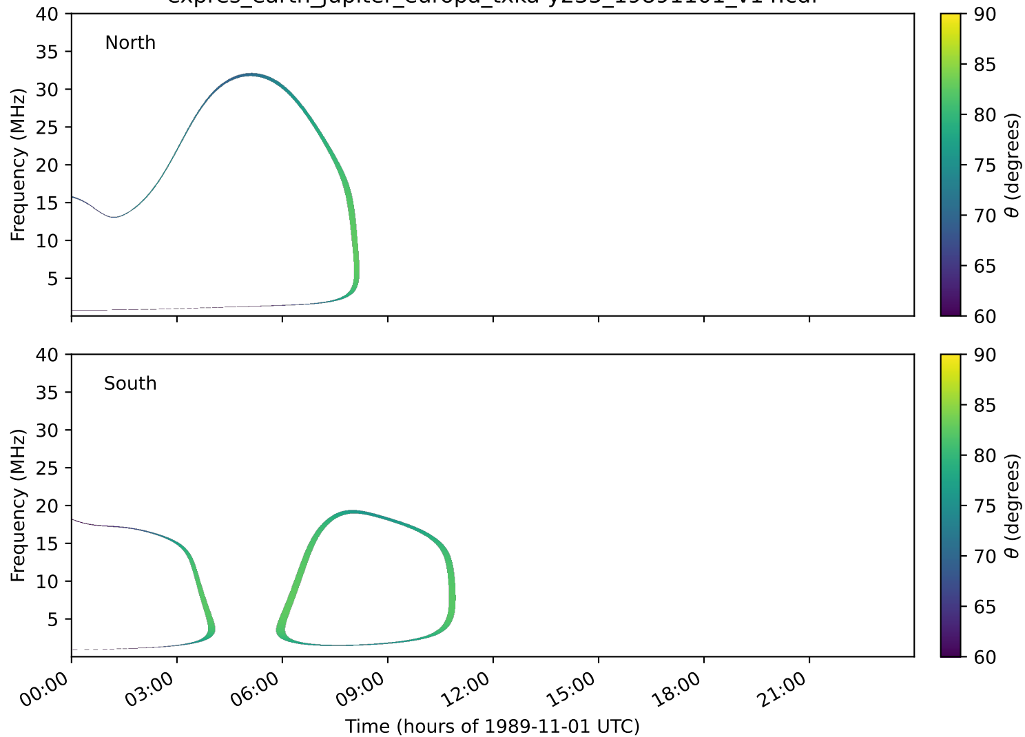
expres_earth_jupiter_europa_txka-y235_19891101_v14.cdf
