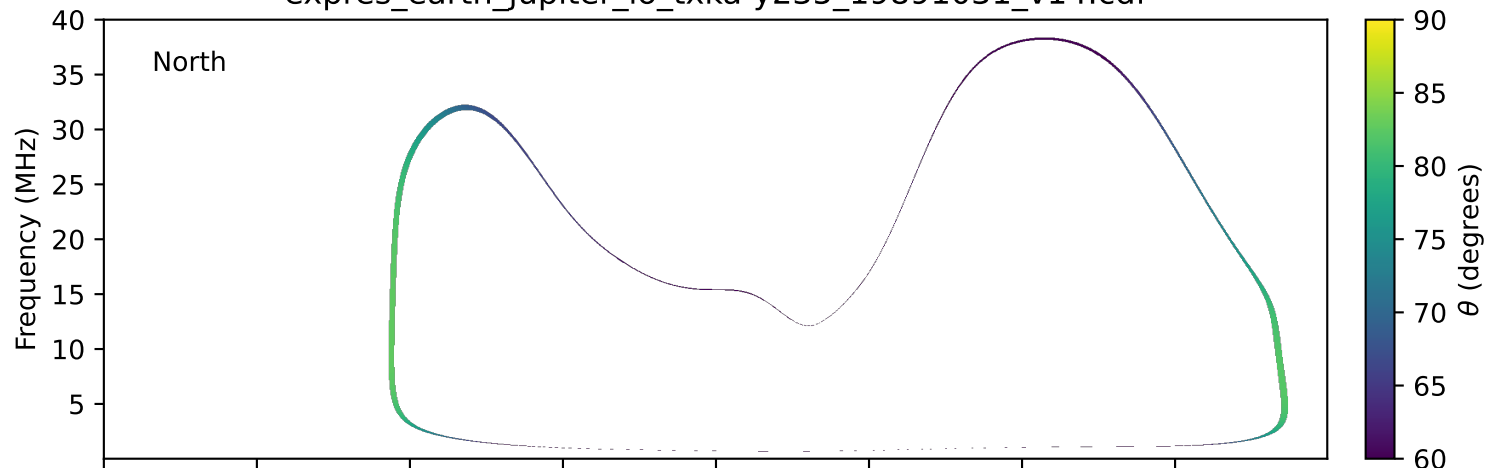
expres_earth_jupiter_io_txka-y235_19891031_v14.cdf
