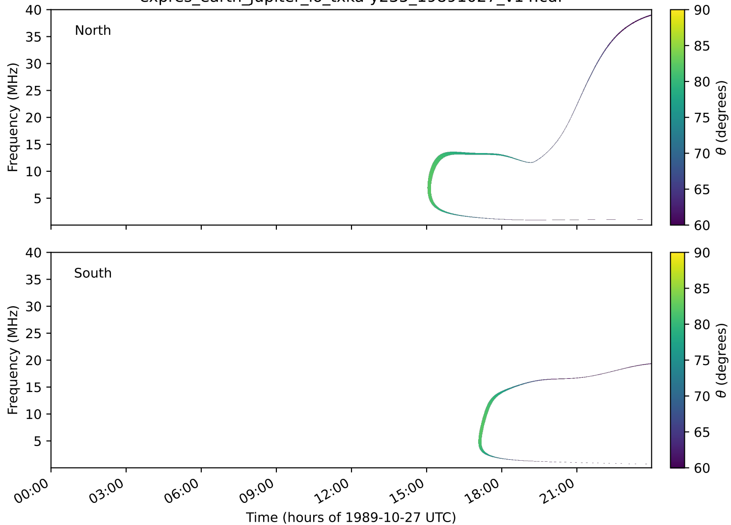
expres_earth_jupiter_io_txka-y235_19891027_v14.cdf
