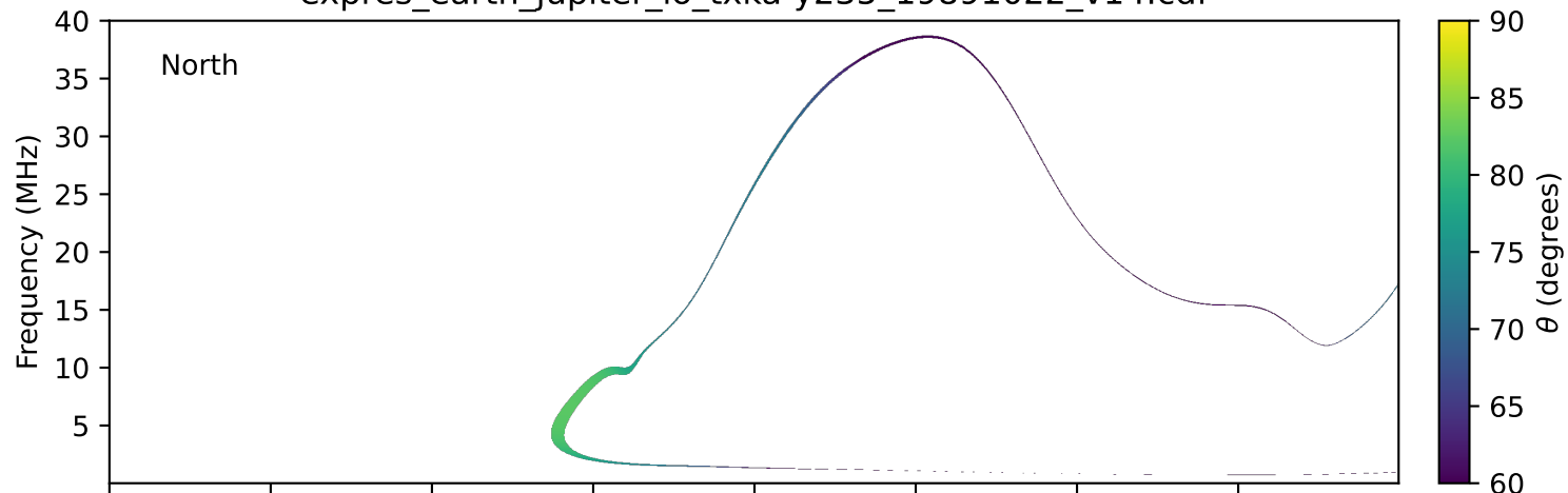
expres_earth_jupiter_io_txka-y235_19891022_v14.cdf
