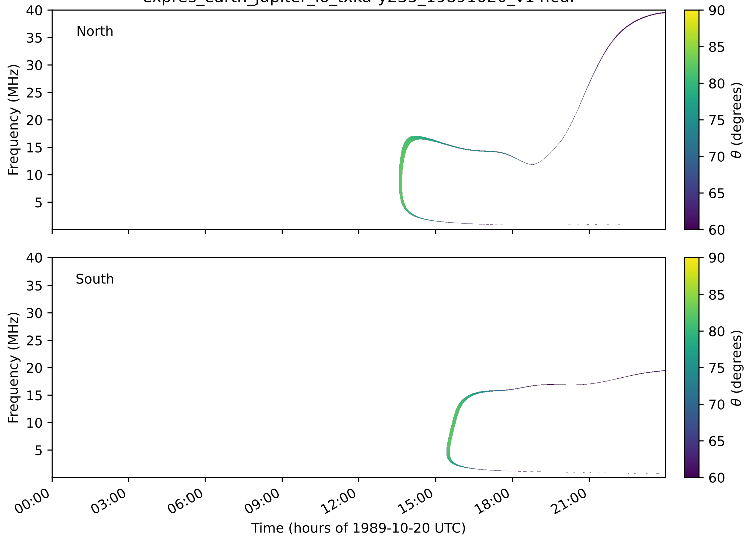
expres_earth_jupiter_io_txka-y235_19891020_v14.cdf
