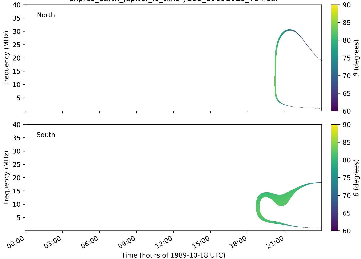
expres_earth_jupiter_io_txka-y235_19891018_v14.cdf
