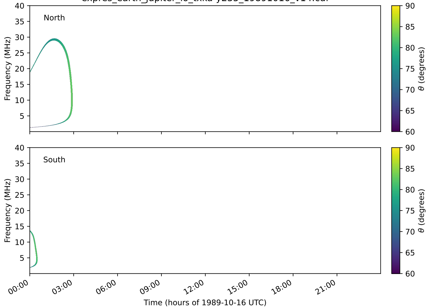
expres_earth_jupiter_io_txka-y235_19891016_v14.cdf
