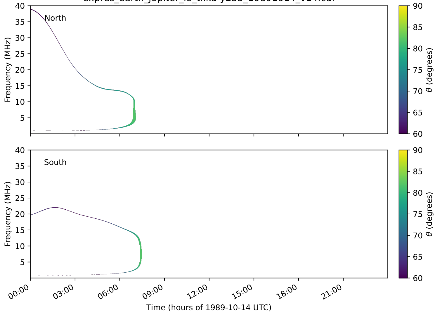
expres_earth_jupiter_io_txka-y235_19891014_v14.cdf
