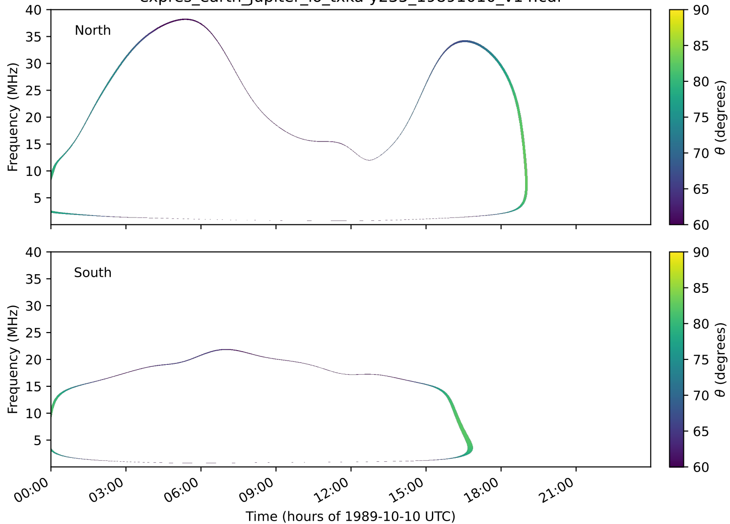
expres_earth_jupiter_io_txka-y235_19891010_v14.cdf
