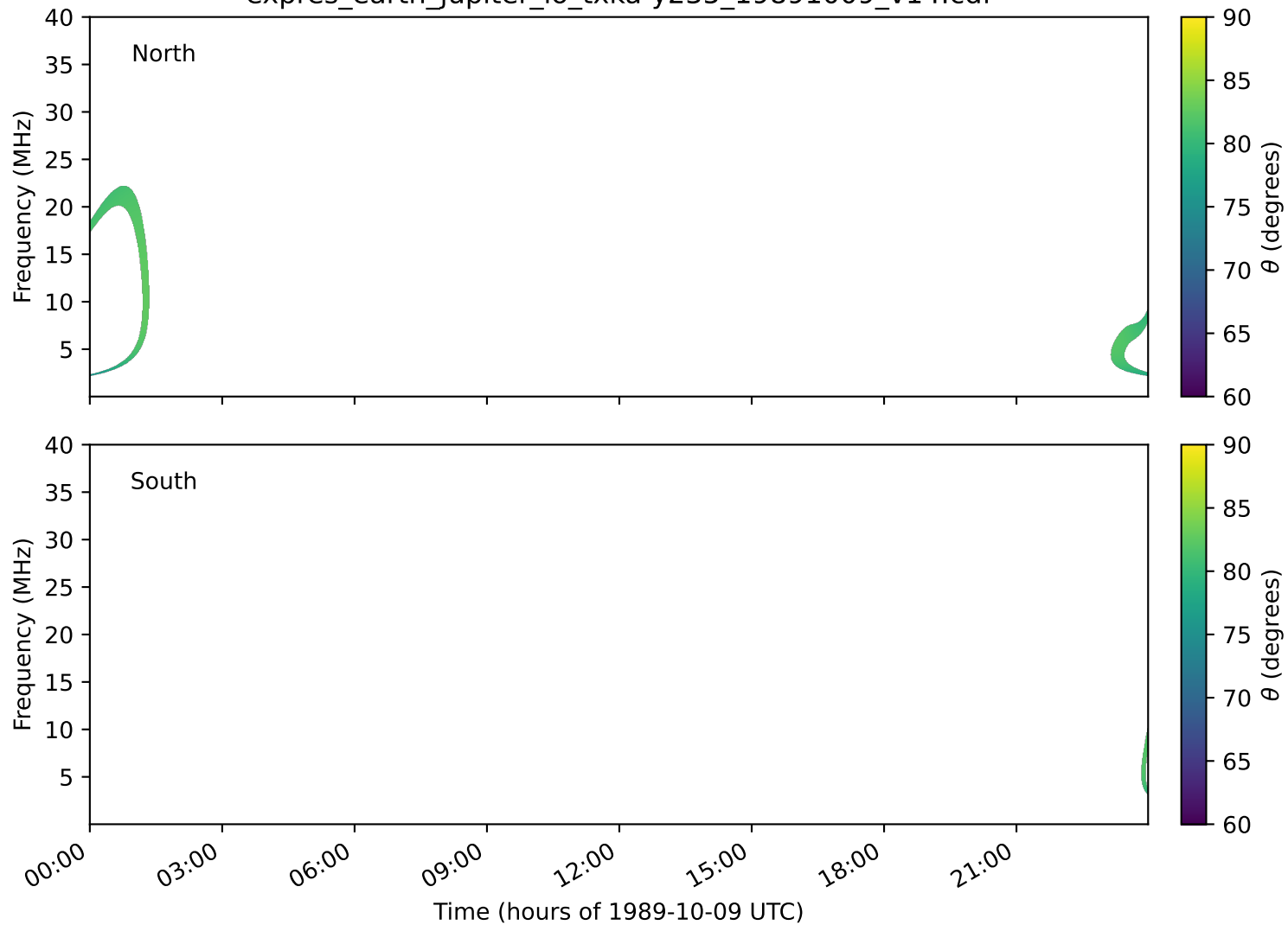
expres_earth_jupiter_io_txka-y235_19891009_v14.cdf
