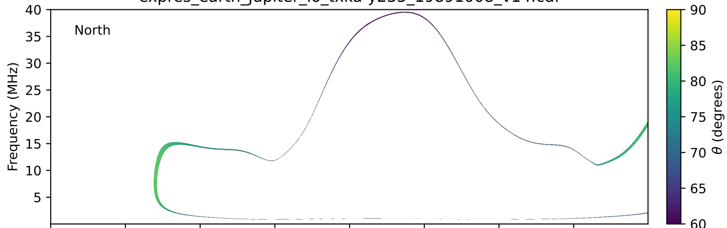
expres_earth_jupiter_io_txka-y235_19891008_v14.cdf
