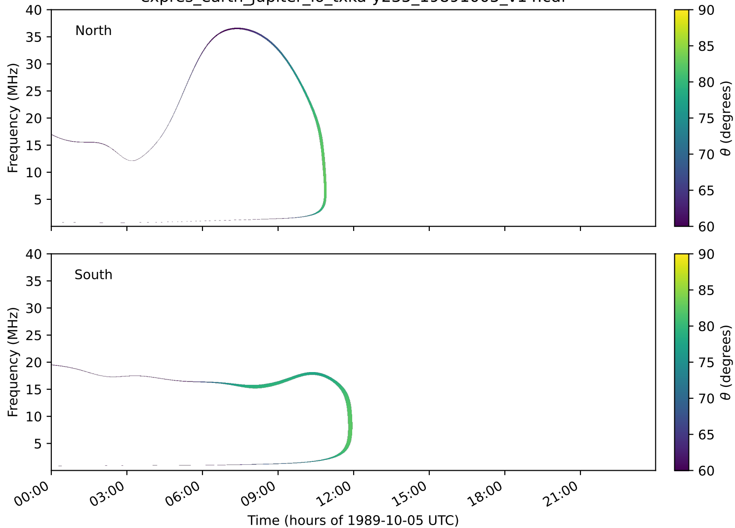
expres_earth_jupiter_io_txka-y235_19891005_v14.cdf
