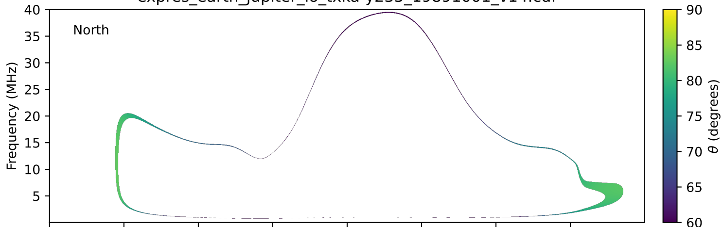
expres_earth_jupiter_io_txka-y235_19891001_v14.cdf
