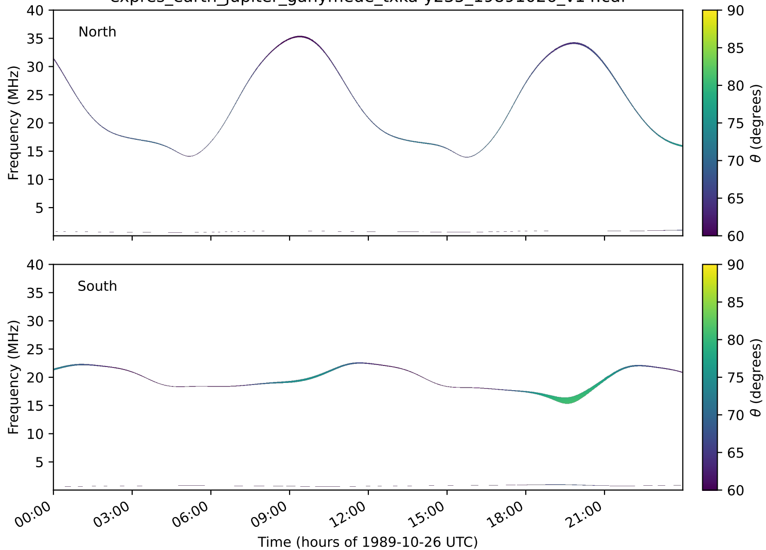
expres_earth_jupiter_ganymede_txka-y235_19891026_v14.cdf
