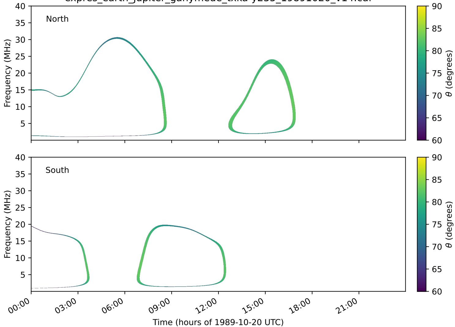
expres_earth_jupiter_ganymede_txka-y235_19891020_v14.cdf
