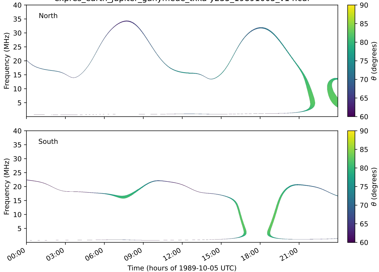
expres_earth_jupiter_ganymede_txka-y235_19891005_v14.cdf
