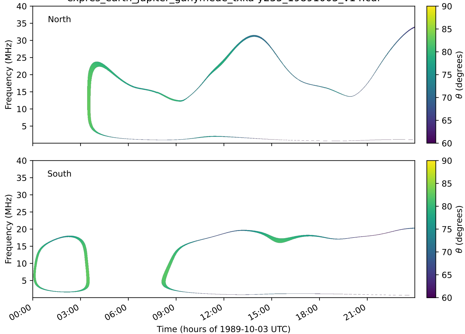
expres_earth_jupiter_ganymede_txka-y235_19891003_v14.cdf
