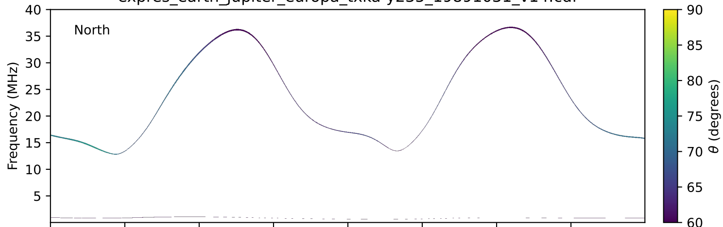
expres_earth_jupiter_europa_txka-y235_19891031_v14.cdf
