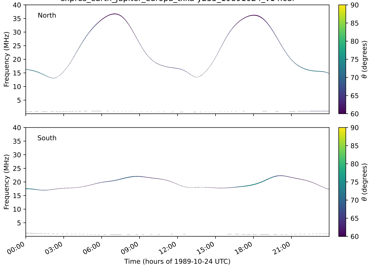
expres_earth_jupiter_europa_txka-y235_19891024_v14.cdf
