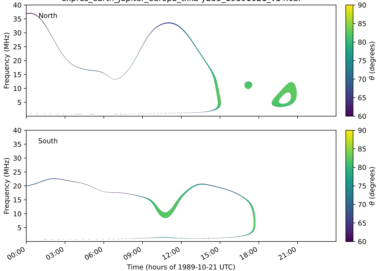
expres_earth_jupiter_europa_txka-y235_19891021_v14.cdf
