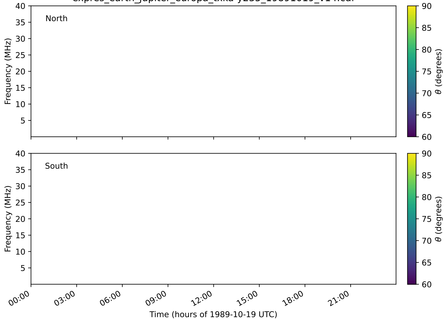
expres_earth_jupiter_europa_txka-y235_19891019_v14.cdf
