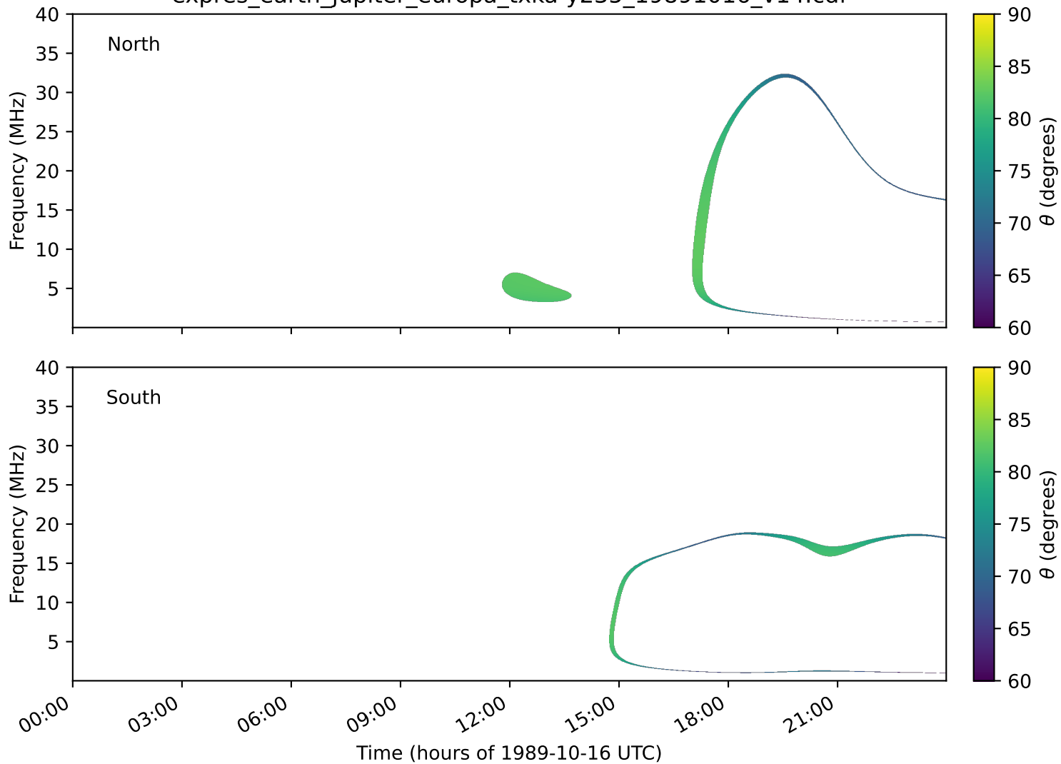
expres_earth_jupiter_europa_txka-y235_19891016_v14.cdf
